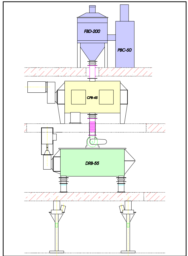
CPB-45 for corrosive rubber reclamation application. Mixer is Kynar® coated carbon steel with Hastelloy components.
