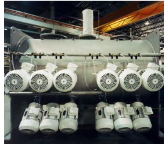
Twelve high speed choppers on this Plow Blender achieve high shear and maximum dispersion.
