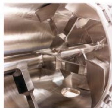
CPB-90 Vacuum Dryer for drying and enhancing the color of organic pigment. Unit has hydraulic drive, tubular load cell base, spherical disc valve, and charge inlet with davit arm.
