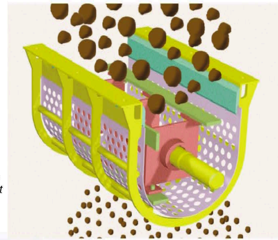
Beater impacts product against screen
